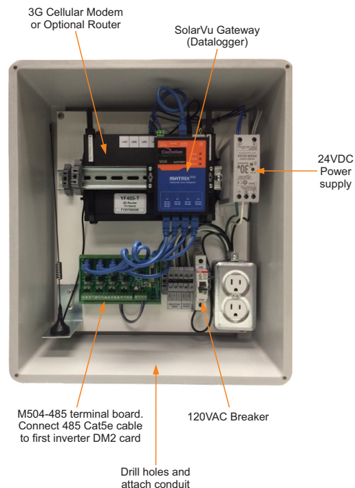
Fig 2 Typical SolarVu enclosure
